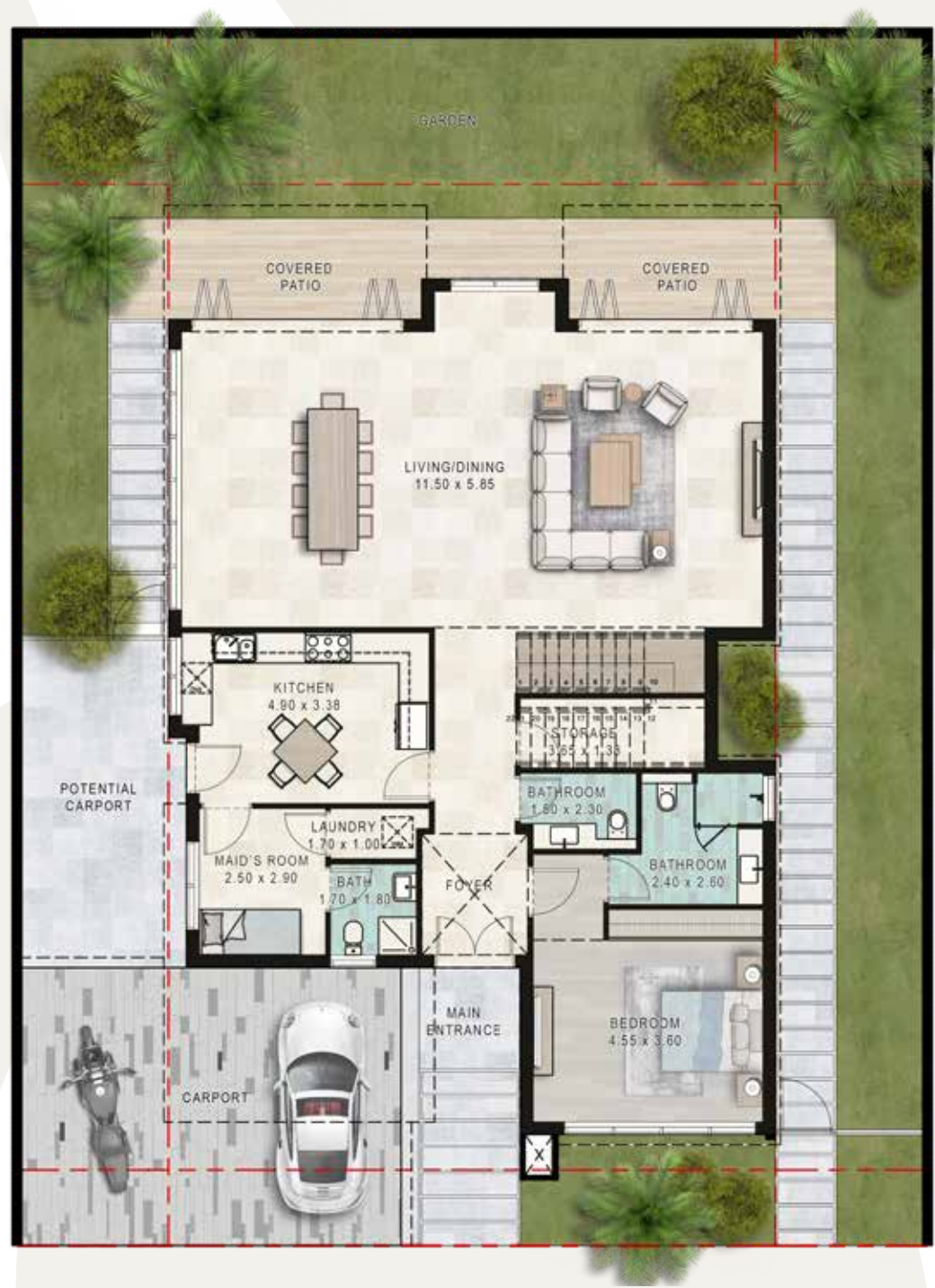
GROUND FLOOR
